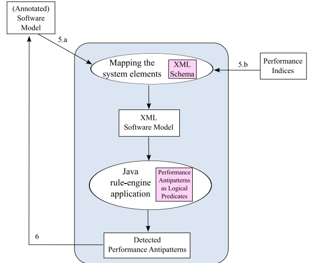
(b) Antipattern-based Results Interpretation & Feedback Generation.
