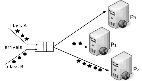
Figure 3. A scenario of the Concurrent Processing Systems antipattern.
