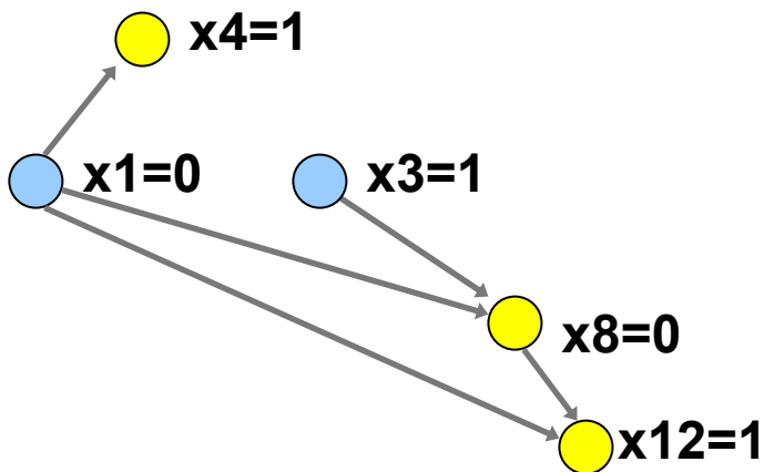
Implication Graph
