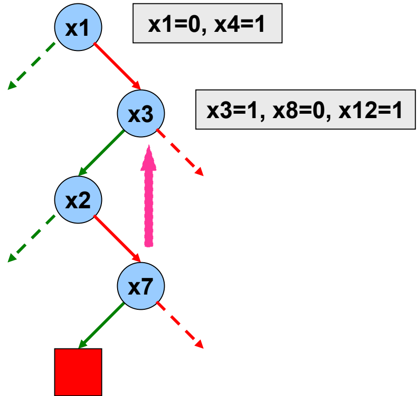
Decision Tree
